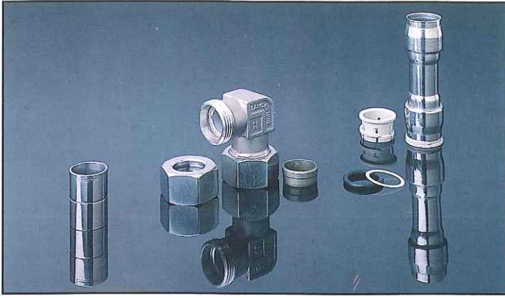
Above: from left to right, capillary, compression and push-in fittings
