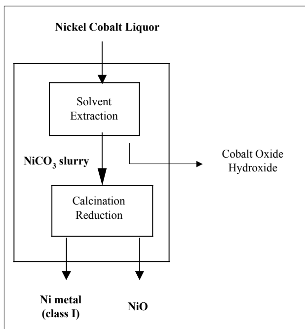
Figure 36 Caron Process: Ni products Production from Nickel Cobalt Liquor
