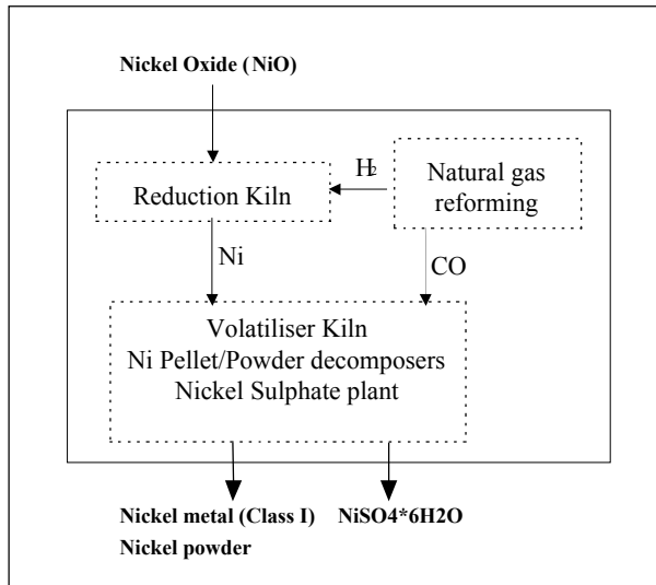
Figure 38 Refining (Pyrometallurgical): Class 1 Ni Production from NiO
