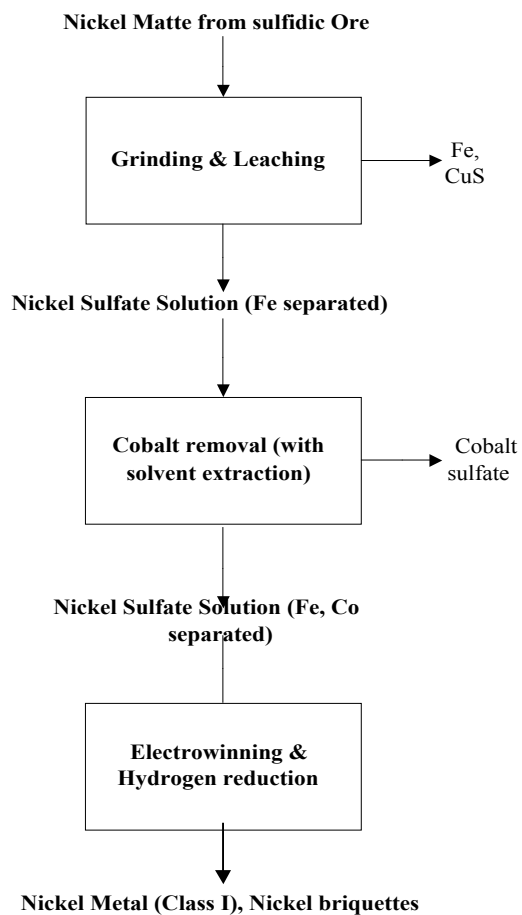
Figure 34 Refining (Hydrosulfidic): Ni Products Production from Nickel Matte
