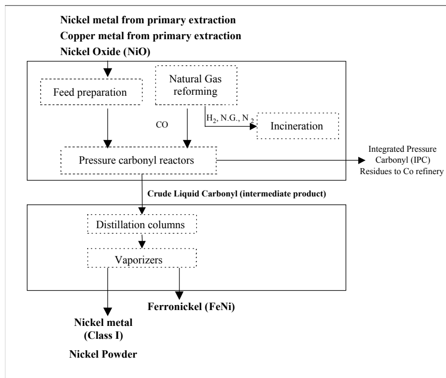
Figure 37 Refining: Class 1 Ni and FeNi Production with Cu/Ni Metallics and NiO (Carbonyl Process)
