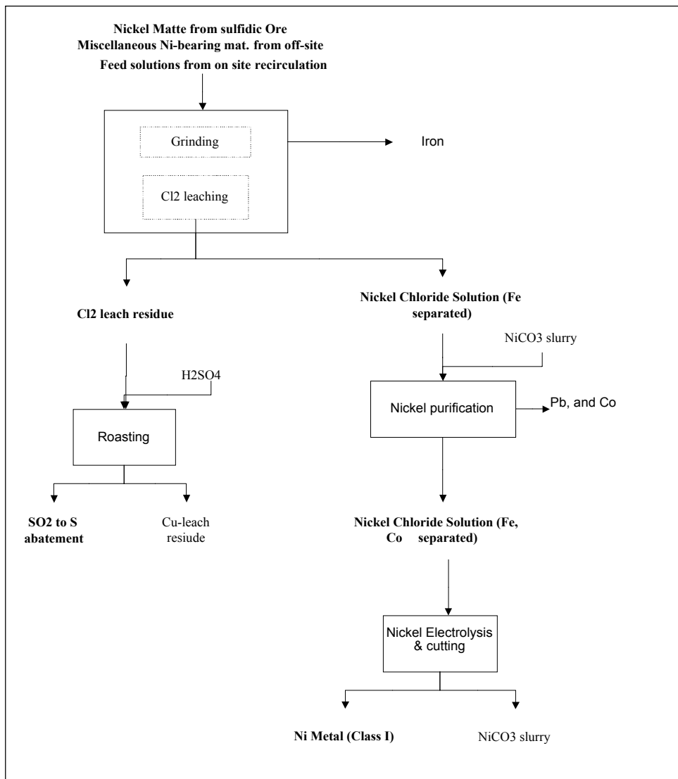
Figure 35 Refining (Hydrosulfidic): Ni Products Production from Various Nickel Feeds
