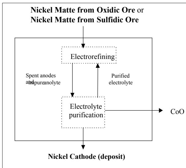
Figure 31 Refining (Hydrosulfidic): Ni Cathode Production from Nickel Matte (Part 1)
