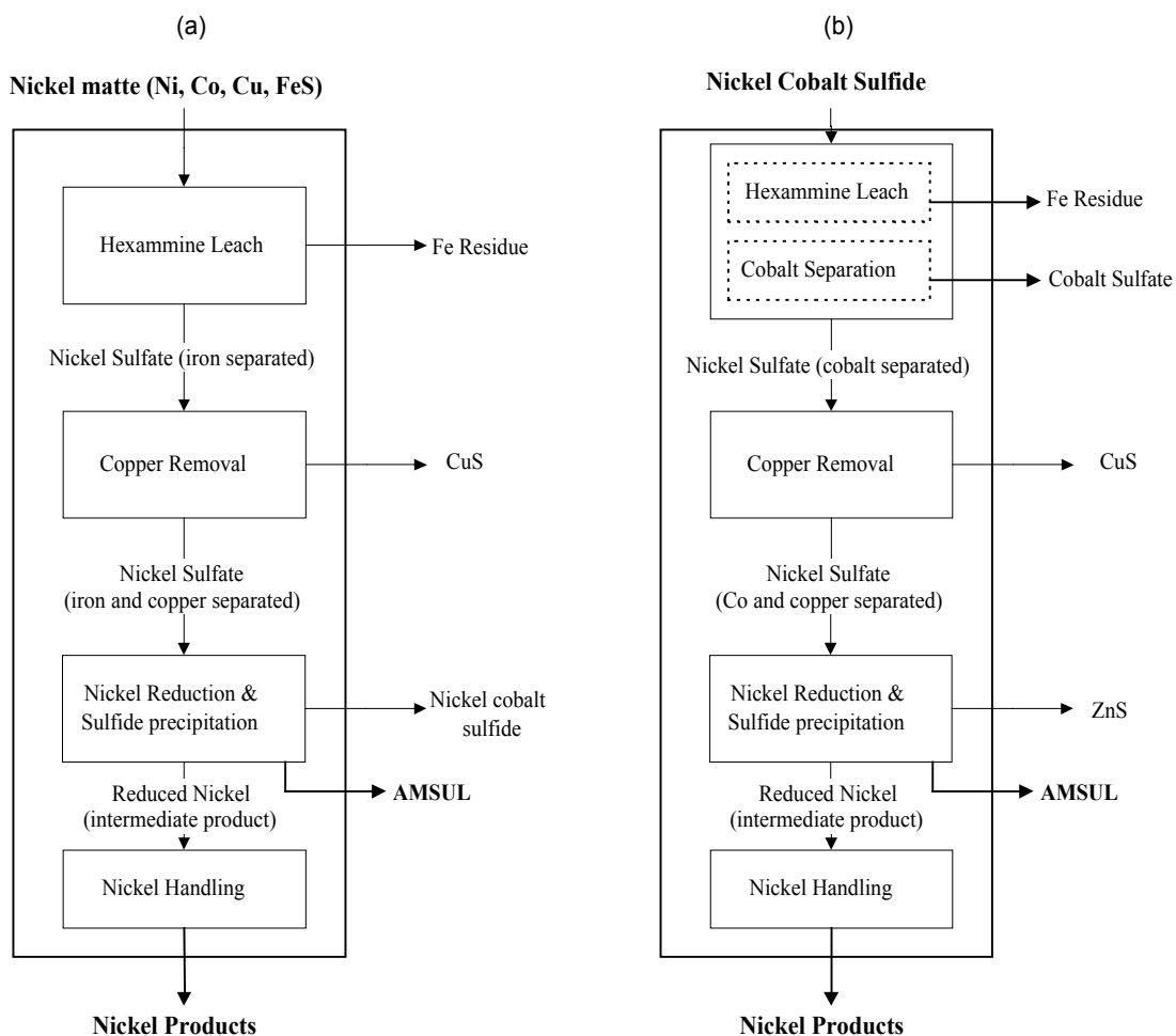
Figure 33a and b Refining (Hydrosulfidic): Ni Products Production from Nickel Cobalt Sulfide and Nickel Matte
