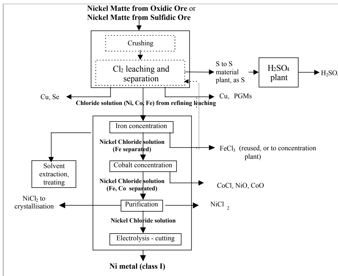
Figure 29 Refining: Class 1 Ni Production from Matte (Integrated Facility)
