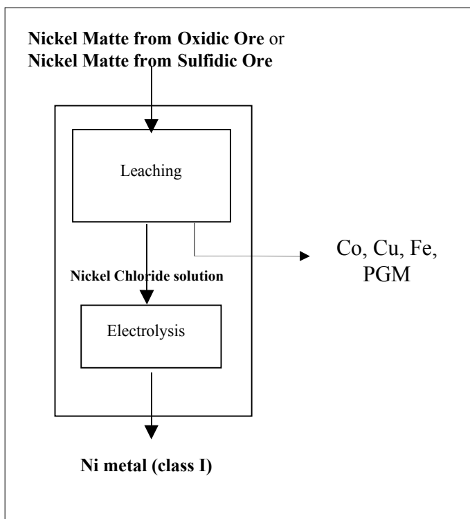
Figure 30 Refining: Class 1 Ni Production from Matte (Less Integrated Facility)
