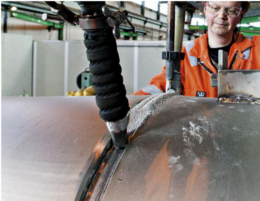
Submerged arc welding. © ESAB Welding & Cutting
